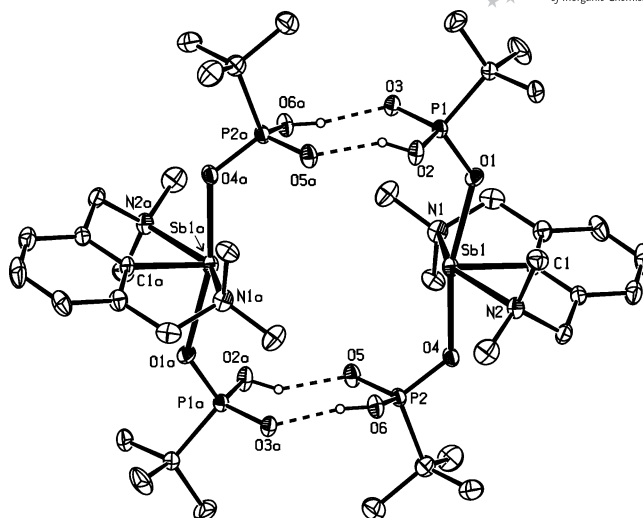
Figure 2. ORTEP diagram of compound 5 with thermal displacement parameters at 30% probability; hydrogen atoms, except those involved in hydrogen bonds, are omitted for clarity. Symmetry operator a = 1 - x, -y, -z . Selected distances [Å] and angles [°]: Sb1–C1 2.092(8), Sb1–N1 2.385(7), Sb1–N2 2.464(8), Sb1–O1 2.204(5), Sb1–O4 2.184(5), O2–O5a 2.495(9), O3–O6a 2.517(8), C1–Sb1–N1 74.6(3), C1–Sb1–N2 74.03, C1–Sb1–O1 81.2(3), C1–Sb1–O4 83.5(3), N1–Sb1–N2 148.3(3), O1–Sb1–O4 164.6(2), O2–H(O2)–O5a 153, O3–H(O6a)–O6a 168.
