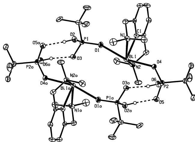
Figure 3. ORTEP diagram of compound 8 with thermal displacement parameters at 30% probability; hydrogen atoms, except those involved in hydrogen bonds, are omitted for clarity. Symmetry operator a = -x, -y, 1 - z . Selected distances [Å] and angles [°]: Bi1–C1 2.177(6), Bi1–N1 2.510(5), Bi1–N2 2.500(5), Bi1–O1 2.353(4), Bi1–O4 2.270(4), O2–O5a 2.553(6), O3–O6a 2.541(6), C1–Bi1–N1 72.6(2), C1–Bi1–N2 73.60(19), C1–Bi1–O1 79.12(19), C1–Bi1–O4 83.62(18), N1–Bi1–N2 146.17(17), O1–Bi1–O4 162.62(14), O2–H(O2)–O5a 168, O3–H(O6a)–O6a 172.
