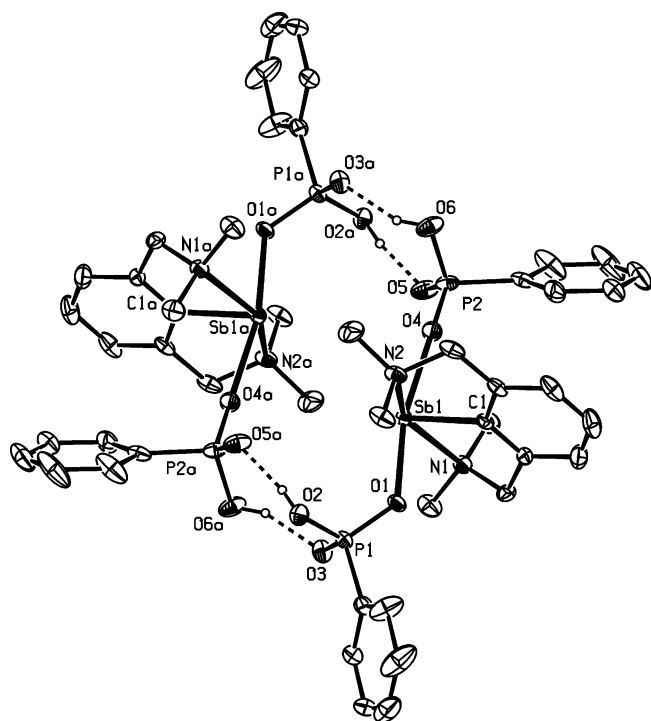
Figure 1. ORTEP diagram of compound 4 with thermal displacement parameters at 30% probability; hydrogen atoms, except those involved in hydrogen bonds, are omitted for clarity. Symmetry operator a = 2 - x, 1 - y, 1 - z . Selected distances [Å] and angles [°]: Sb1–C1 2.103(3), Sb1–N1 2.454(3), Sb1–N2 2.396(3), Sb1–O1 2.198(3), Sb1–O4 2.229(3), O2–O5a 2.477(2), O3–O6a 2.508(5), C1–Sb1–N1 74.31(13), C1–Sb1–N2 74.73(13), C1–Sb1–O1 83.11(12), C1–Sb1–O4 81.94(12), N1–Sb1–N2 149.04(12), O1–Sb1–O4 164.93(10), O2–H(O2)–O5a 170, O3–H(O6a)–O6a 156.
