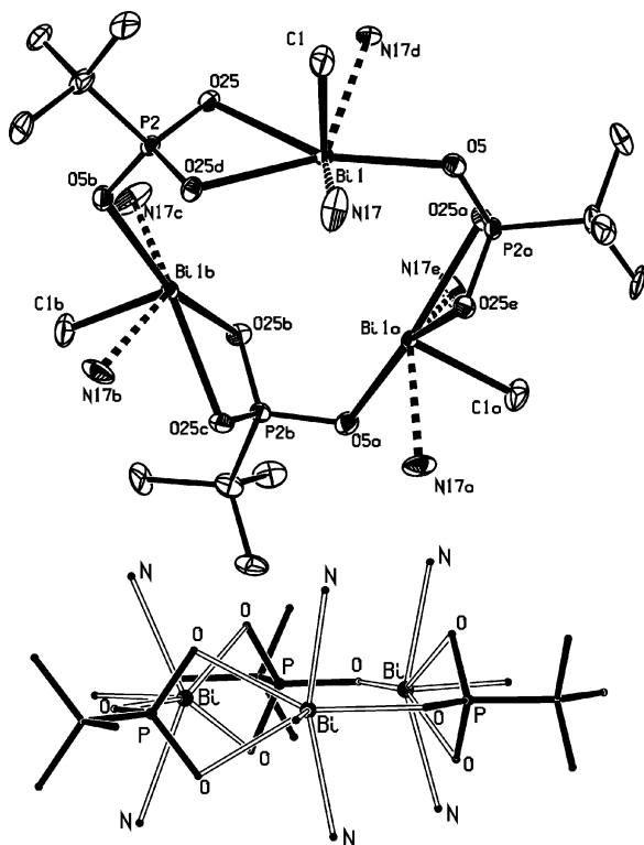
Figure 4. ORTEP diagram of compound 9 with thermal displacement parameters at 30% probability and view of the central ring system. The disordered ligands (except the nitrogen donor atoms and the ipso carbon atoms) and the hydrogen atoms are omitted for clarity. Symmetry operators a = 1 - y, x - y, z ; b = 1 - x + y, 1 - x, z ; c = 1 - x + y, 1 - y, 1/2 - z ; d = x, y, 1/2 - z ; e = 1 - y, x - y, 1/2 - z . Selected distances [Å] and angles [°]: Bi1–C1 2.178(11), Bi1–N17 2.60(2), Bi1–O5 2.313(17), Bi1–O25 2.518(8), C1–Bi1–N17 71.4(6), C1–Bi1–O5 89.8(5), C1–Bi1–O25 88.5(3), N17–Bi1–N17d 136.2(8), N17–Bi1–O5 78.7(4), N17–Bi1–O25d 73.1(5).
